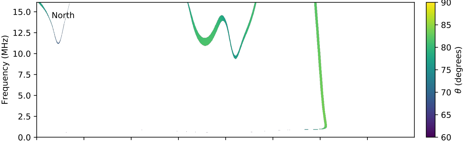
expres_cassini_jupiter_europa_isaac_lossc-wid1deg_3kev_20030705_v01.cdf
