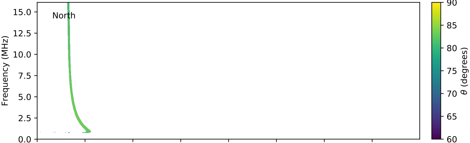
expres_cassini_jupiter_europa_isaac_lossc-wid1deg_3kev_20030702_v01.cdf
