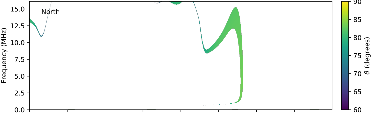
expres_cassini_jupiter_io_isaac_lossc-wid1deg_3kev_20030630_v01.cdf
