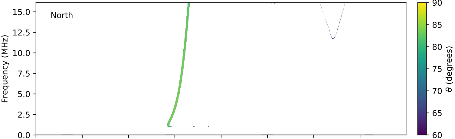
expres_cassini_jupiter_io_isaac_lossc-wid1deg_3kev_20030626_v01.cdf
