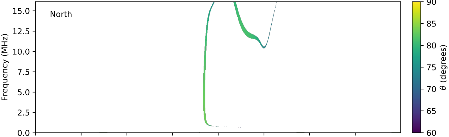
expres_cassini_jupiter_io_isaac_lossc-wid1deg_3kev_20030617_v01.cdf
