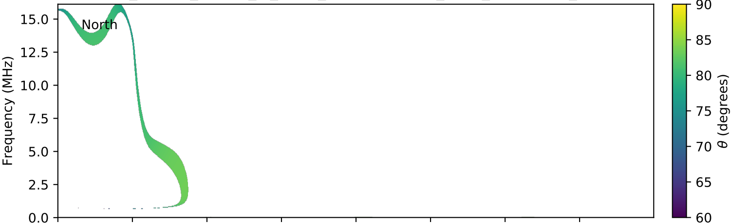
expres_cassini_jupiter_io_isaac_lossc-wid1deg_3kev_20030611_v01.cdf
