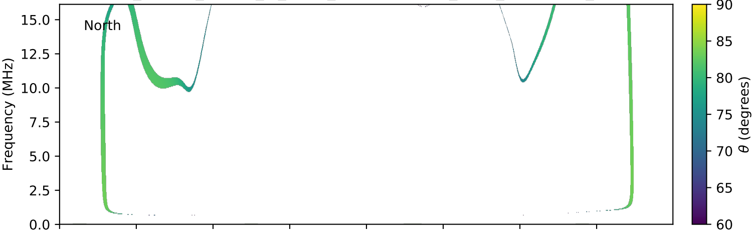
expres_cassini_jupiter_io_isaac_lossc-wid1deg_3kev_20030605_v01.cdf
