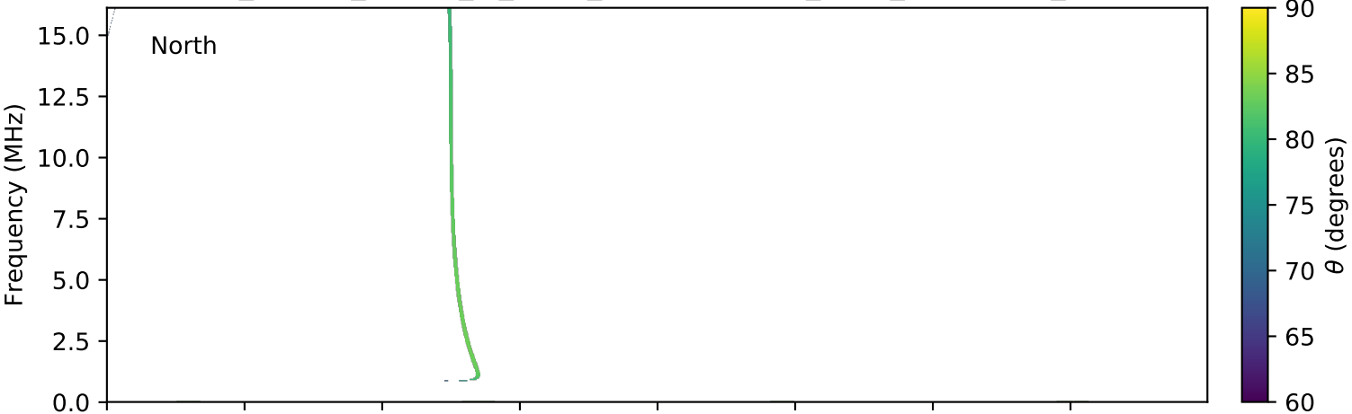
expres_cassini_jupiter_io_isaac_lossc-wid1deg_3kev_20030602_v01.cdf
