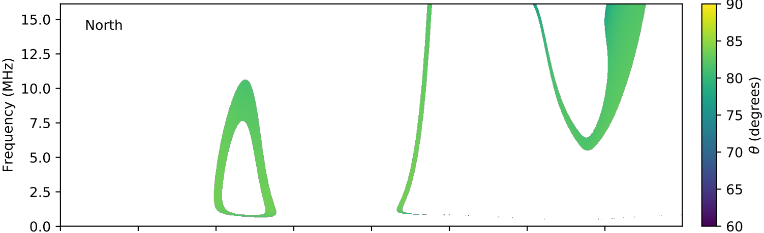
expres_cassini_jupiter_ganymede_isaac_lossc-wid1deg_3kev_20030630_v01.cdf
