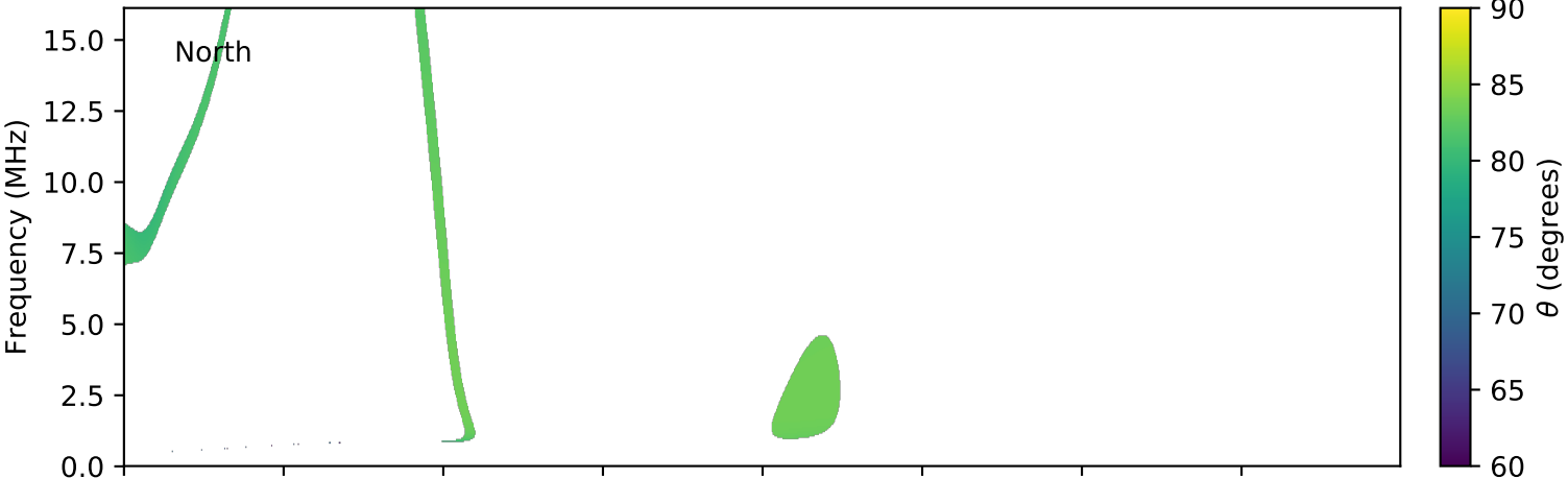
expres_cassini_jupiter_ganymede_isaac_lossc-wid1deg_3kev_20030626_v01.cdf
