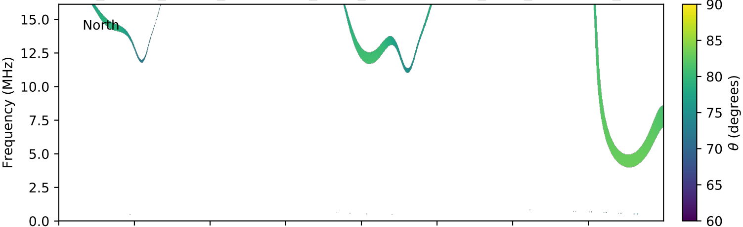
expres_cassini_jupiter_ganymede_isaac_lossc-wid1deg_3kev_20030625_v01.cdf
