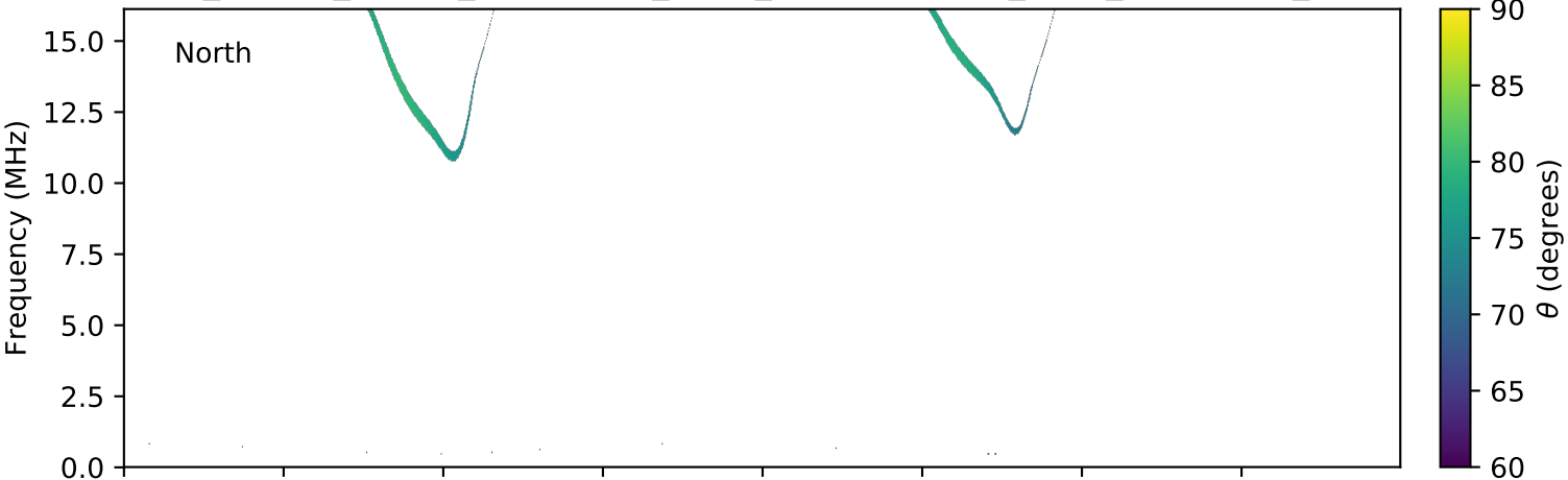
expres_cassini_jupiter_ganymede_isaac_lossc-wid1deg_3kev_20030624_v01.cdf
