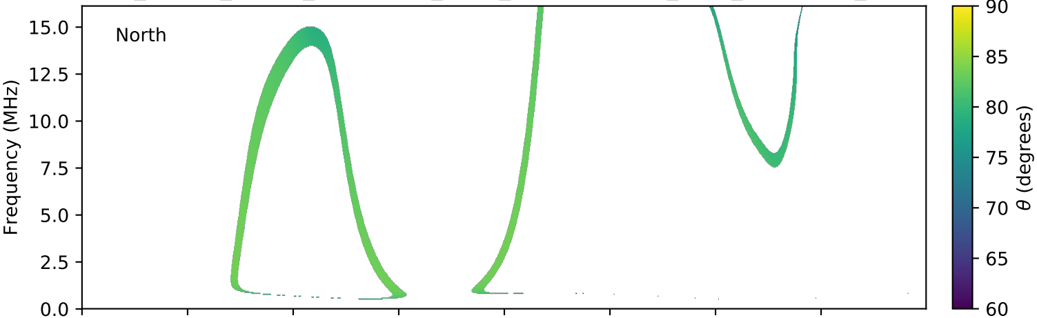
expres_cassini_jupiter_ganymede_isaac_lossc-wid1deg_3kev_20030623_v01.cdf
