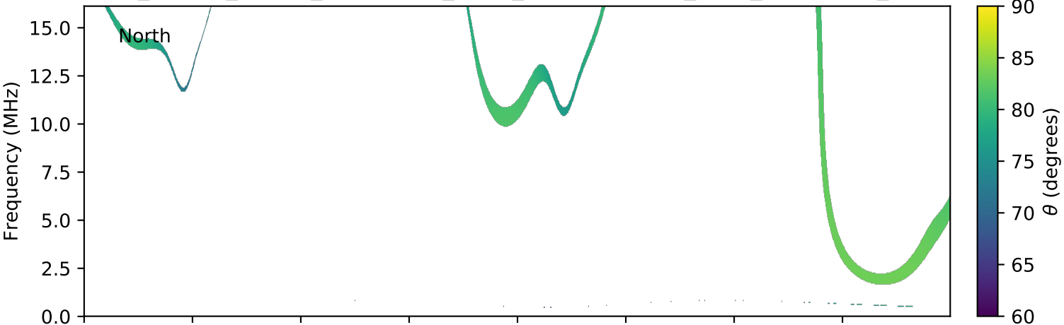
expres_cassini_jupiter_ganymede_isaac_lossc-wid1deg_3kev_20030618_v01.cdf
