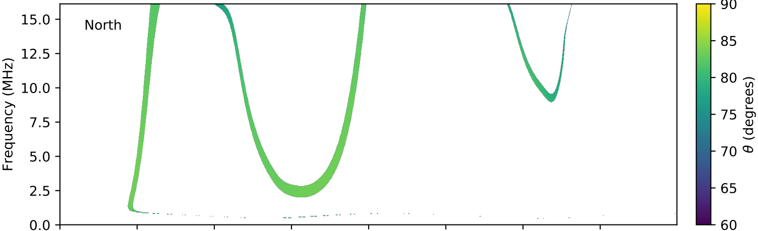
expres_cassini_jupiter_ganymede_isaac_lossc-wid1deg_3kev_20030616_v01.cdf
