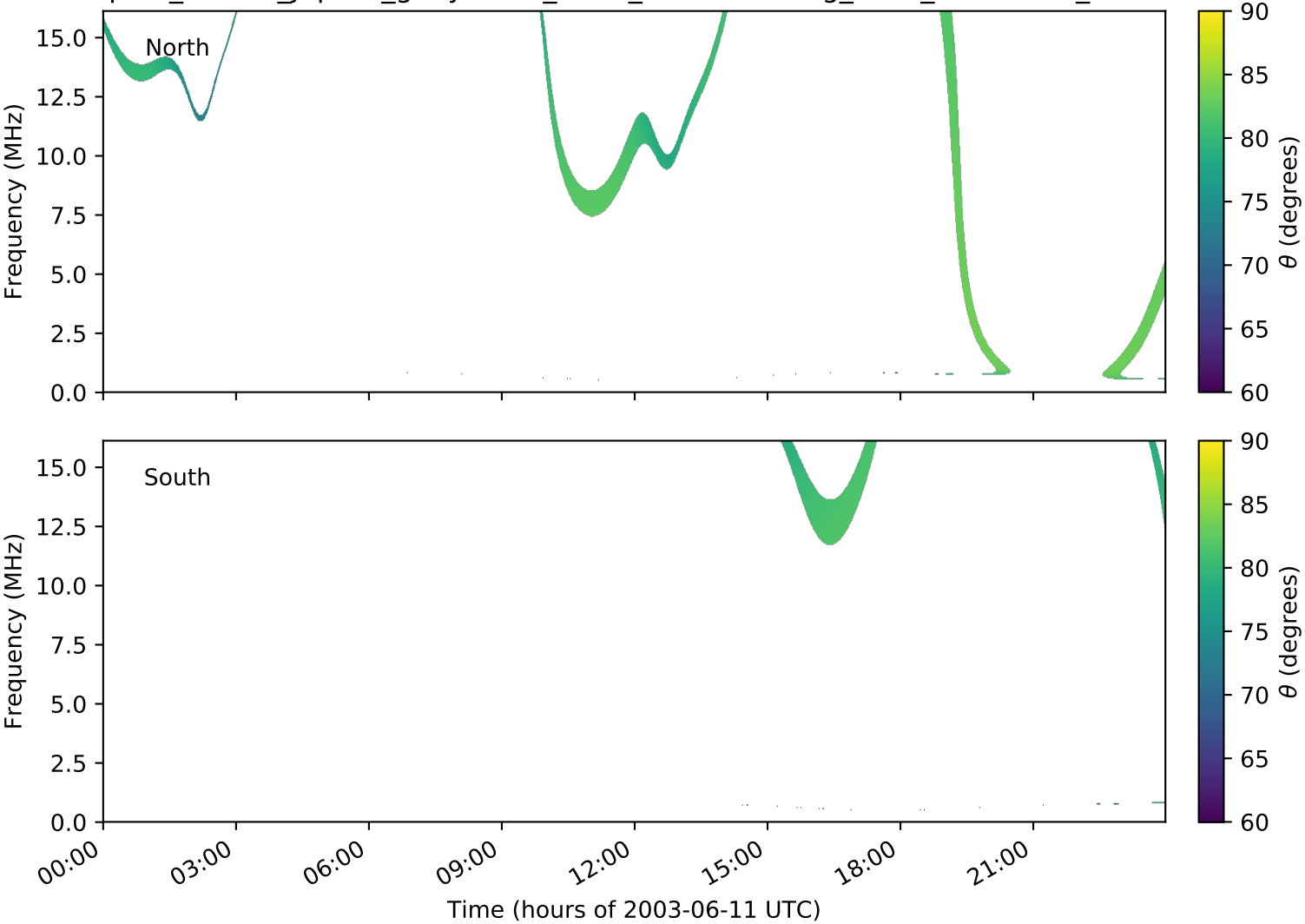
expres_cassini_jupiter_ganymede_isaac_lossc-wid1deg_3kev_20030611_v01.cdf
