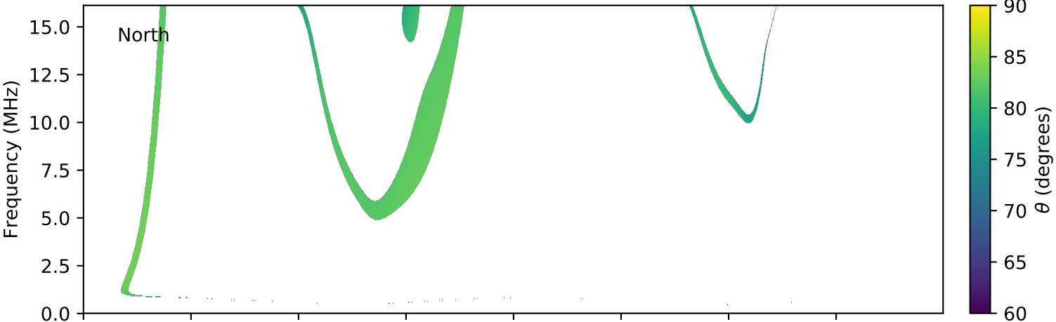
expres_cassini_jupiter_ganymede_isaac_lossc-wid1deg_3kev_20030609_v01.cdf
