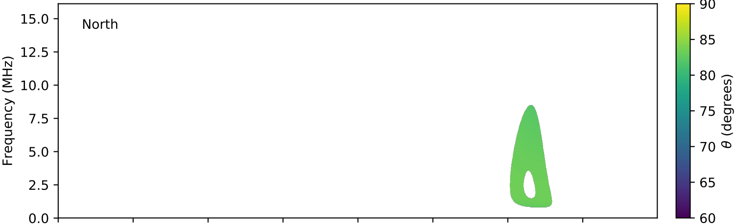
expres_cassini_jupiter_ganymede_isaac_lossc-wid1deg_3kev_20030608_v01.cdf
