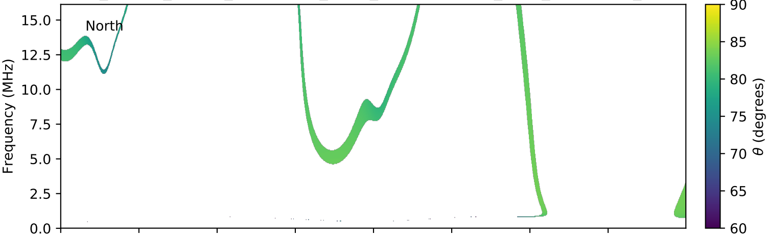
expres_cassini_jupiter_ganymede_isaac_lossc-wid1deg_3kev_20030604_v01.cdf
