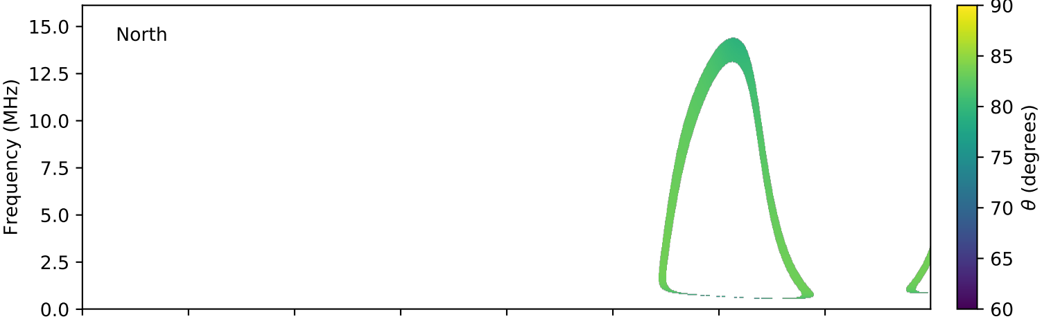
expres_cassini_jupiter_ganymede_isaac_lossc-wid1deg_3kev_20030601_v01.cdf
