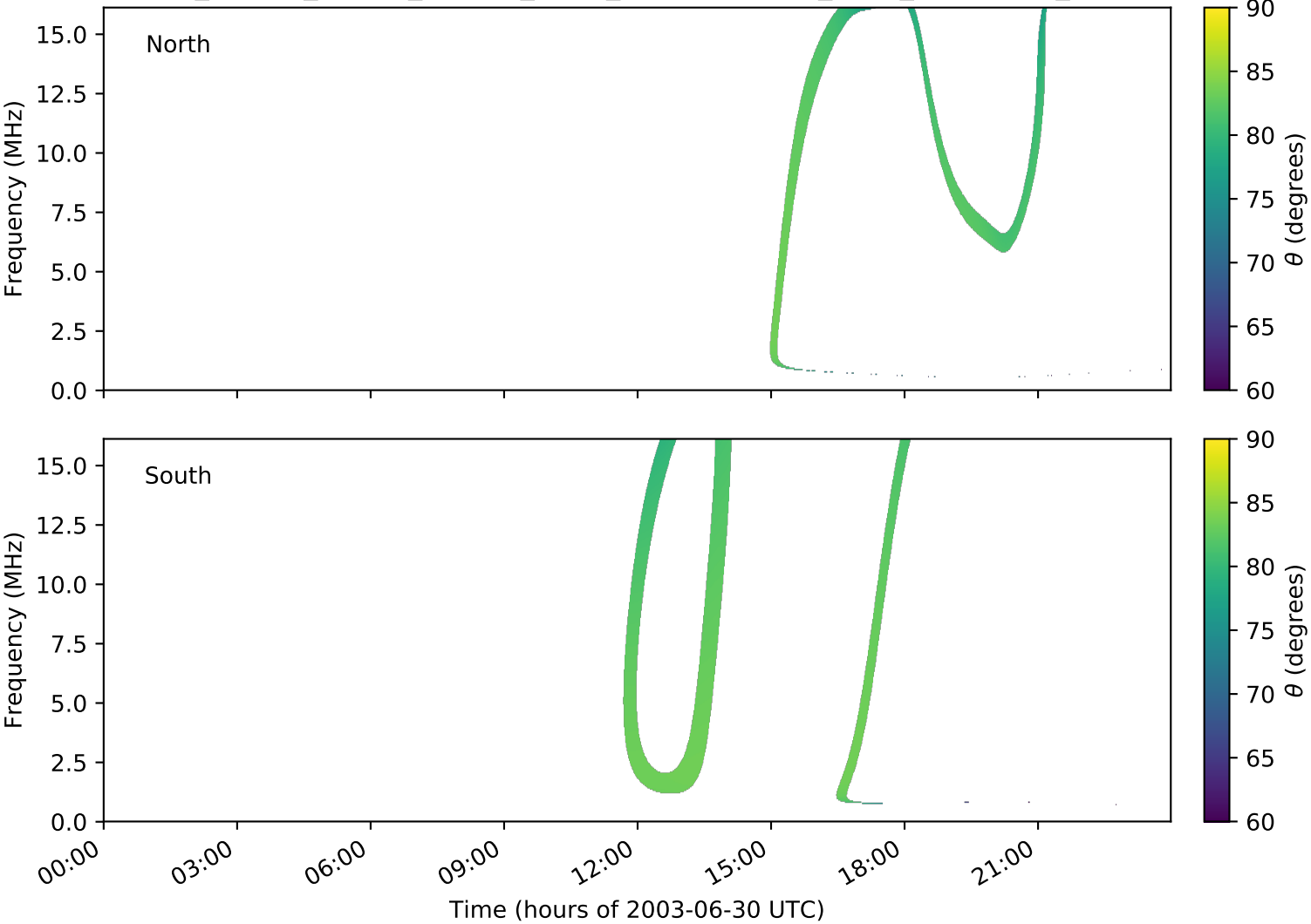
expres_cassini_jupiter_europa_isaac_lossc-wid1deg_3kev_20030630_v01.cdf
