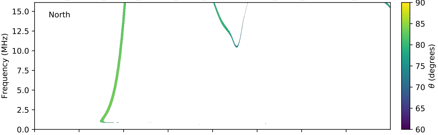
expres_cassini_jupiter_europa_isaac_lossc-wid1deg_3kev_20030627_v01.cdf
