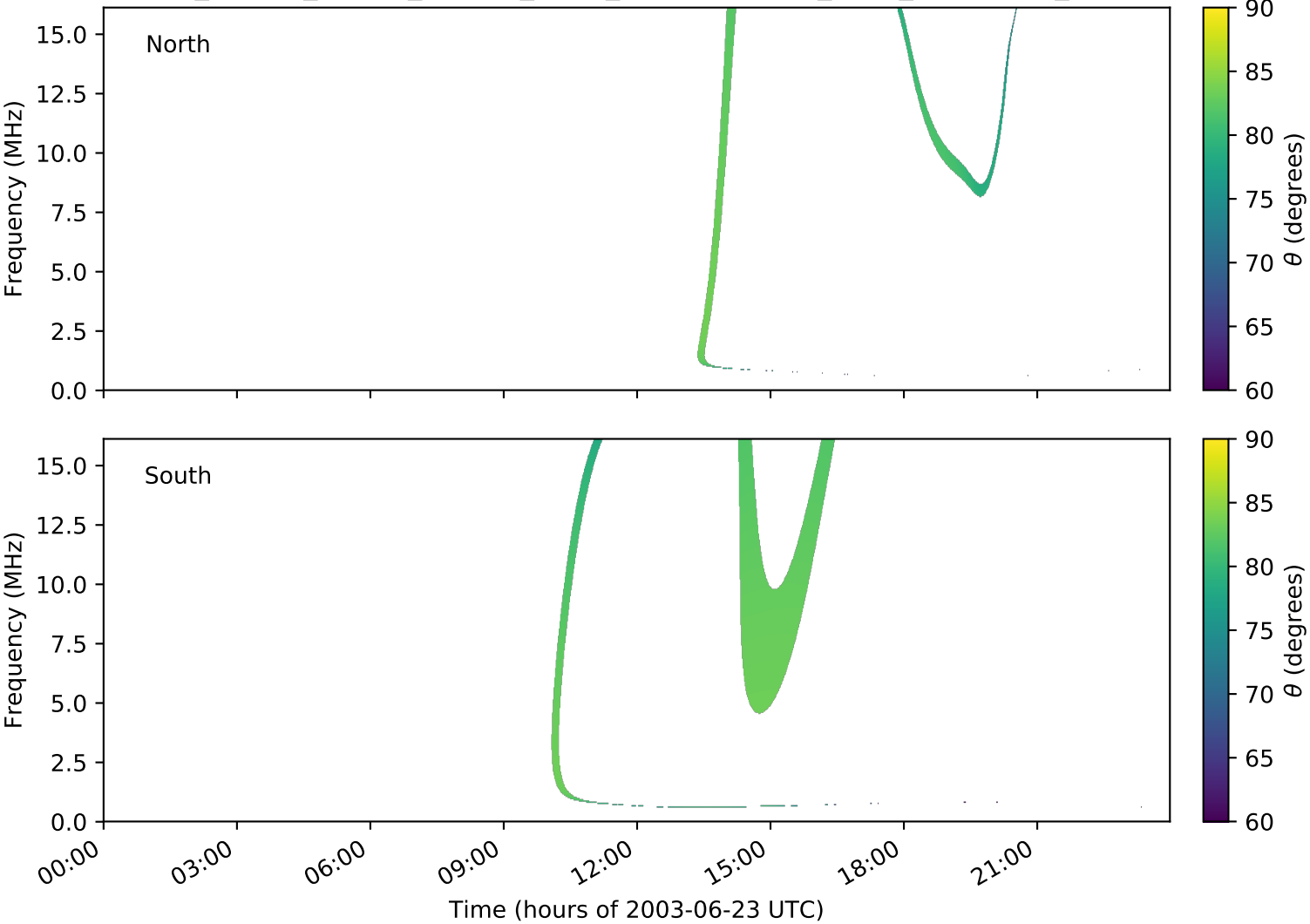
expres_cassini_jupiter_europa_isaac_lossc-wid1deg_3kev_20030623_v01.cdf
