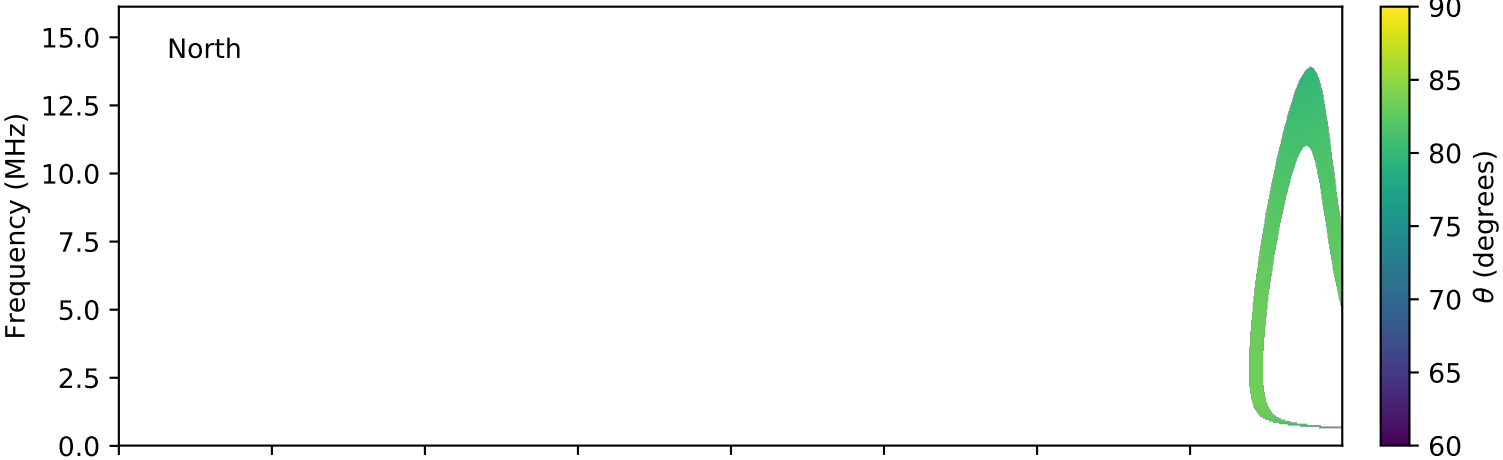
expres_cassini_jupiter_europa_isaac_lossc-wid1deg_3kev_20030619_v01.cdf
