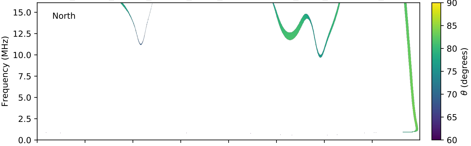
expres_cassini_jupiter_europa_isaac_lossc-wid1deg_3kev_20030617_v01.cdf
