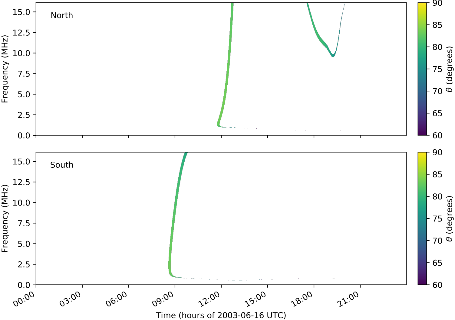
expres_cassini_jupiter_europa_isaac_lossc-wid1deg_3kev_20030616_v01.cdf
