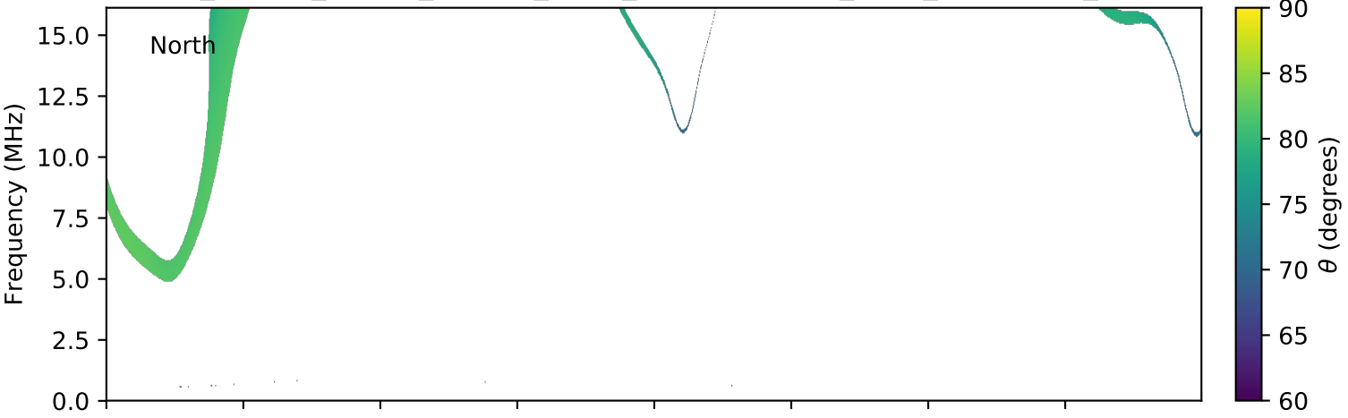
expres_cassini_jupiter_europa_isaac_lossc-wid1deg_3kev_20030613_v01.cdf
