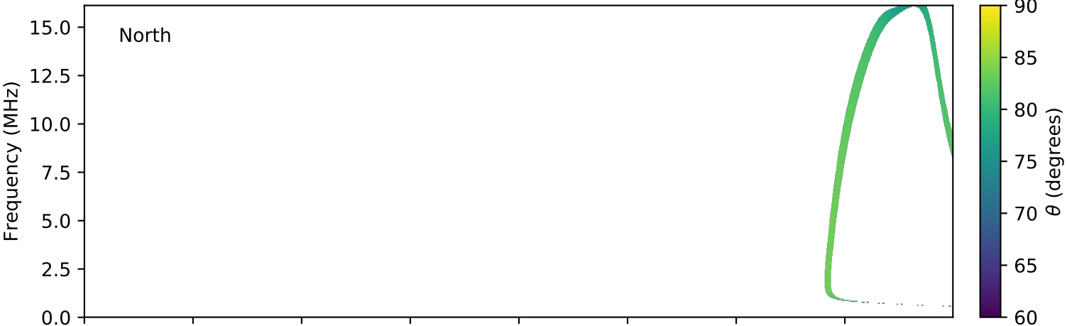
expres_cassini_jupiter_europa_isaac_lossc-wid1deg_3kev_20030612_v01.cdf
