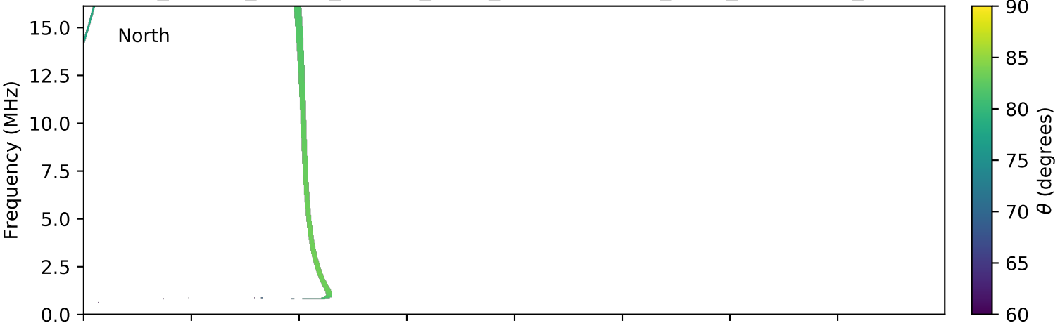
expres_cassini_jupiter_europa_isaac_lossc-wid1deg_3kev_20030607_v01.cdf
