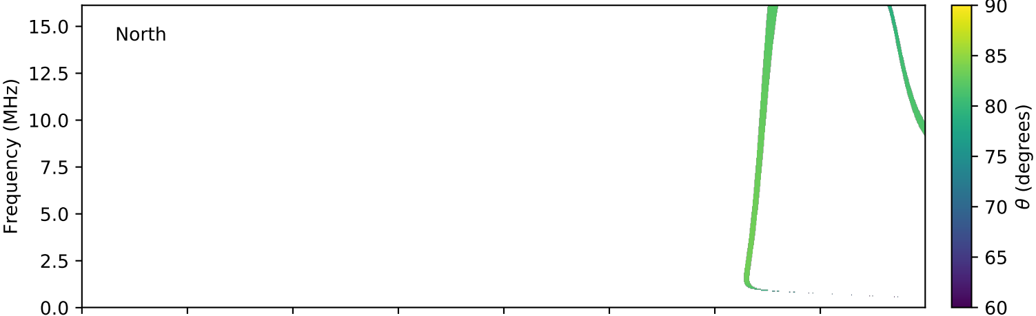
expres_cassini_jupiter_europa_isaac_lossc-wid1deg_3kev_20030605_v01.cdf
