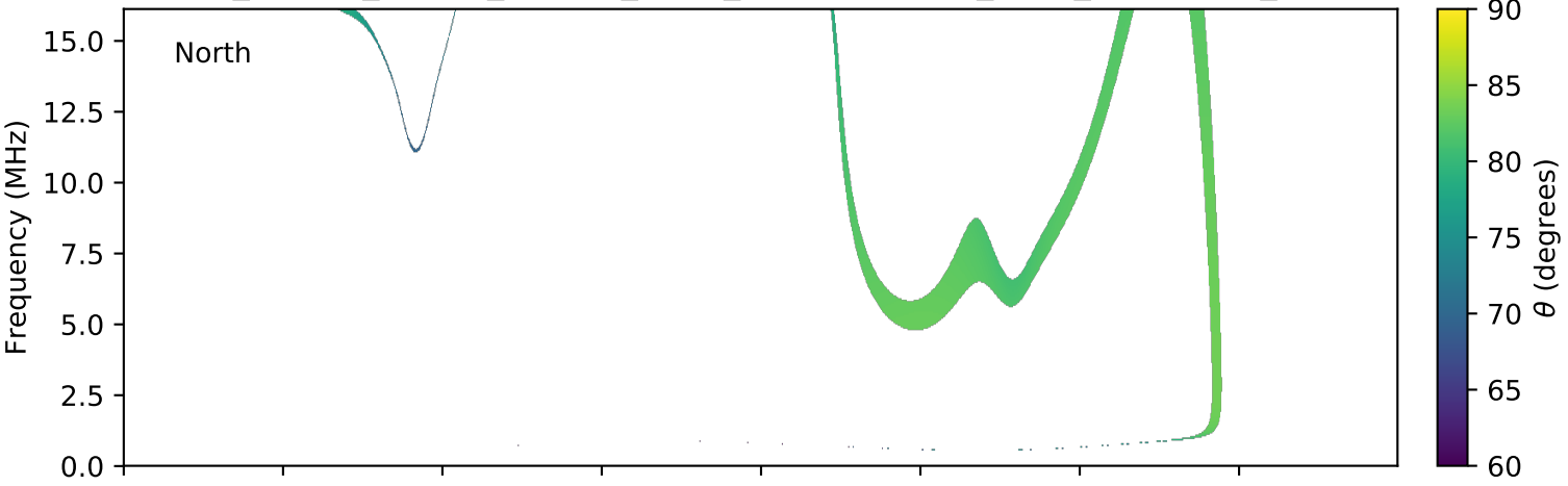
expres_cassini_jupiter_europa_isaac_lossc-wid1deg_3kev_20030603_v01.cdf
