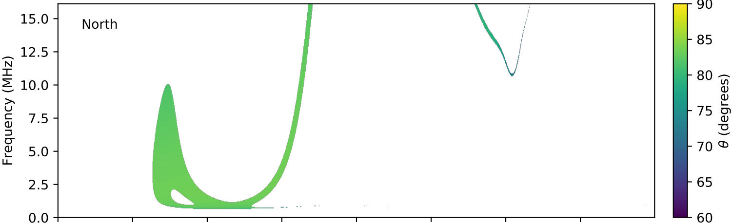
expres_cassini_jupiter_europa_isaac_lossc-wid1deg_3kev_20030602_v01.cdf
