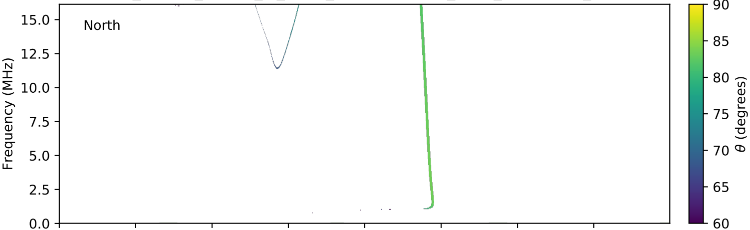
expres_cassini_jupiter_io_isaac_lossc-wid1deg_3kev_20030531_v01.cdf
