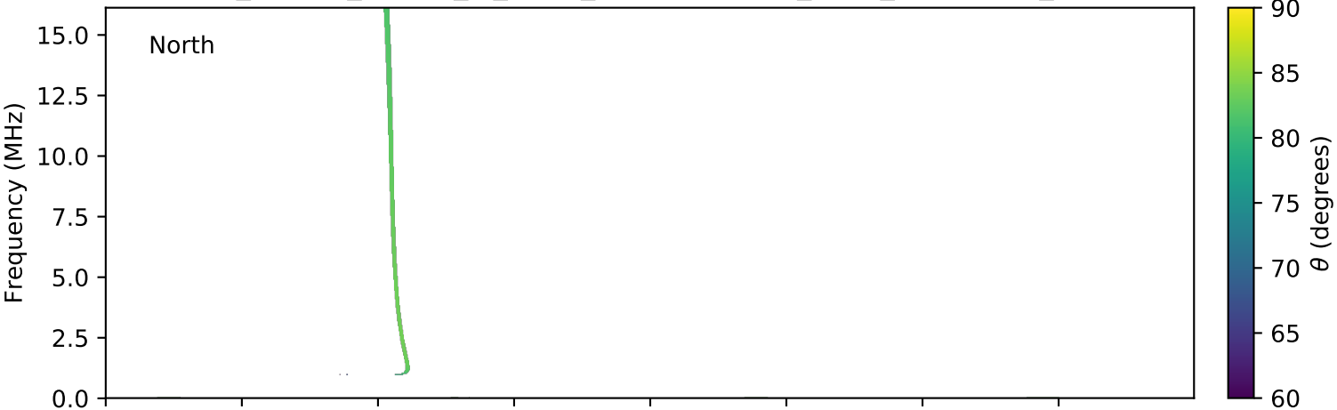
expres_cassini_jupiter_io_isaac_lossc-wid1deg_3kev_20030526_v01.cdf
