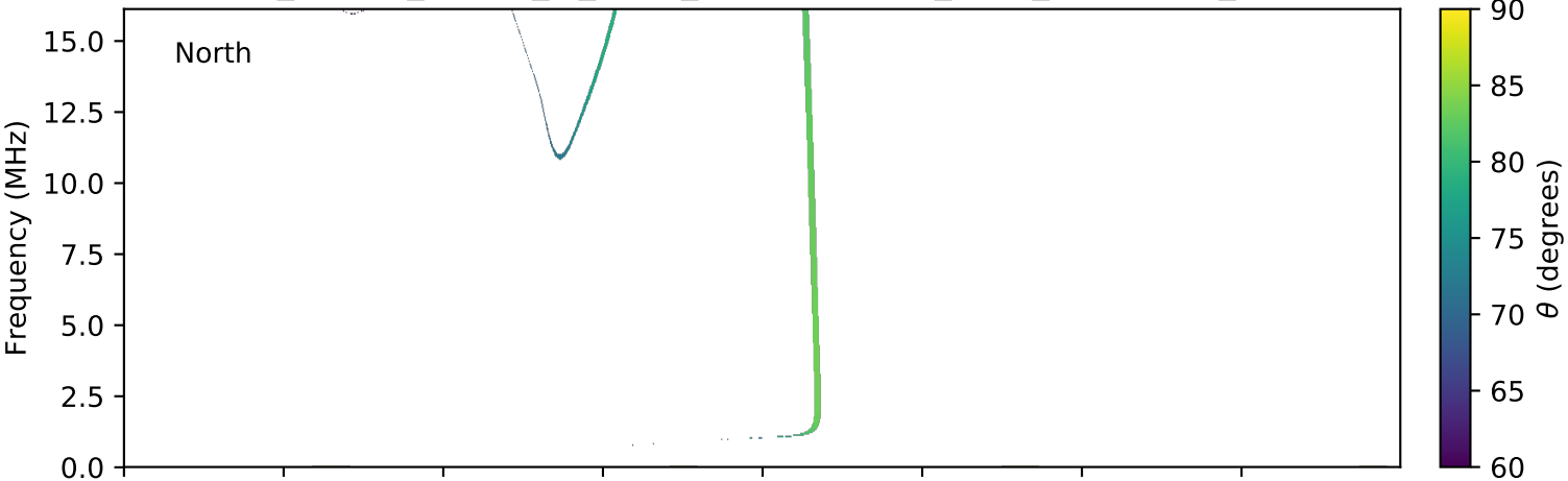
expres_cassini_jupiter_io_isaac_lossc-wid1deg_3kev_20030524_v01.cdf
