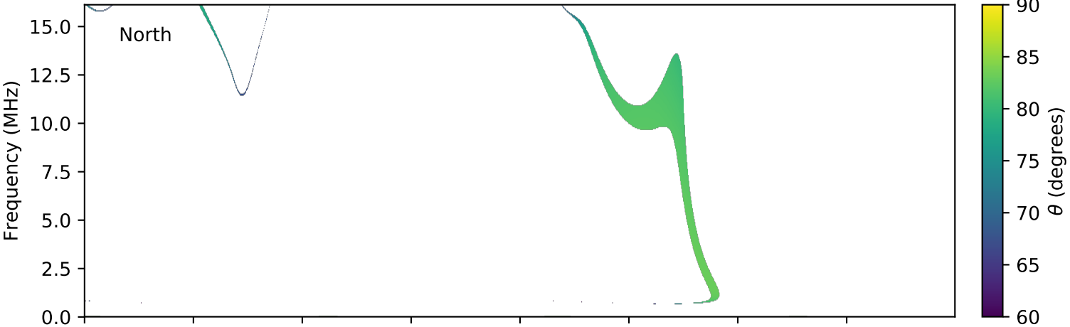
expres_cassini_jupiter_io_isaac_lossc-wid1deg_3kev_20030522_v01.cdf
