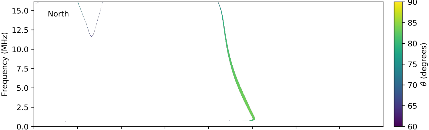
expres_cassini_jupiter_io_isaac_lossc-wid1deg_3kev_20030515_v01.cdf
