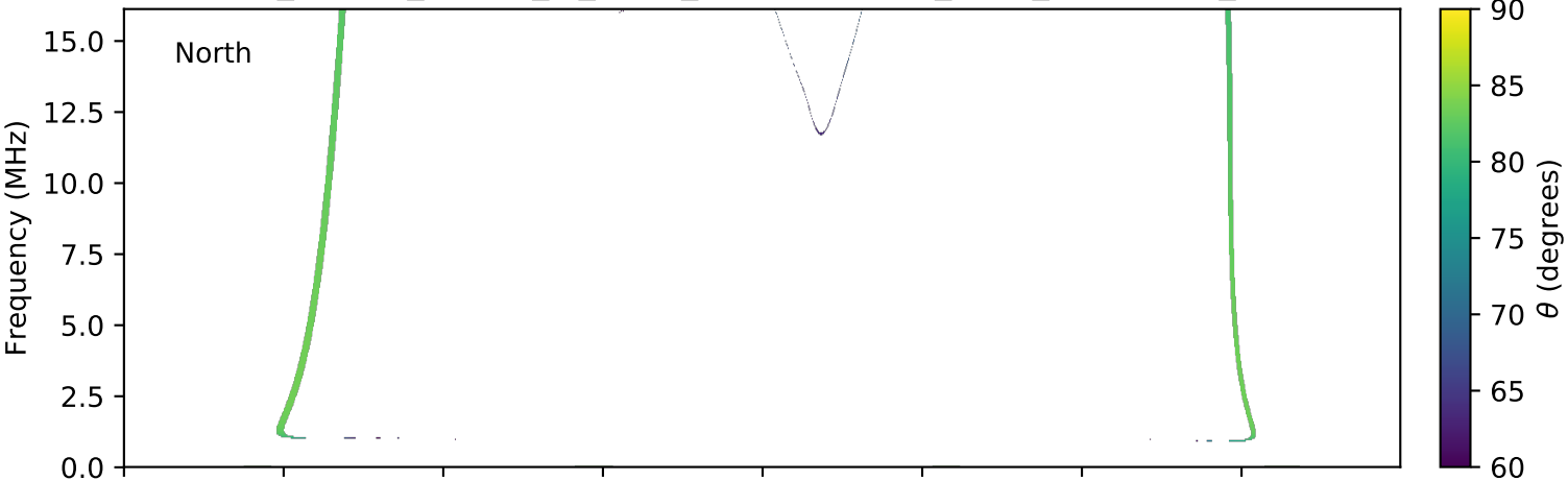
expres_cassini_jupiter_io_isaac_lossc-wid1deg_3kev_20030513_v01.cdf
