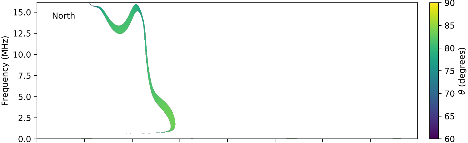
expres_cassini_jupiter_io_isaac_lossc-wid1deg_3kev_20030510_v01.cdf
