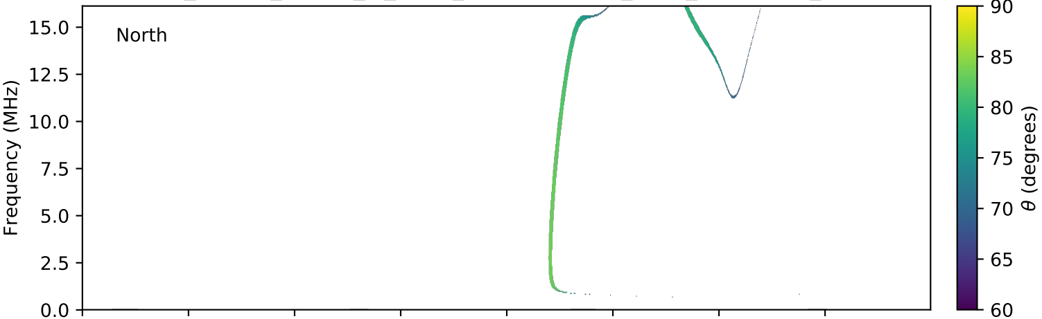
expres_cassini_jupiter_io_isaac_lossc-wid1deg_3kev_20030509_v01.cdf
