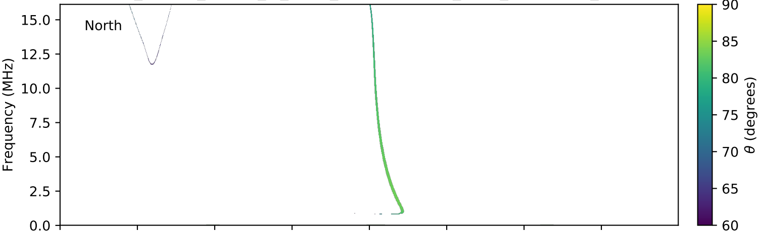
expres_cassini_jupiter_io_isaac_lossc-wid1deg_3kev_20030508_v01.cdf
