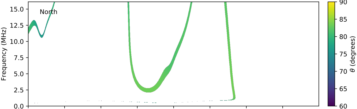
expres_cassini_jupiter_ganymede_isaac_lossc-wid1deg_3kev_20030528_v01.cdf
