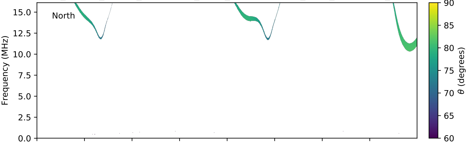
expres_cassini_jupiter_ganymede_isaac_lossc-wid1deg_3kev_20030527_v01.cdf
