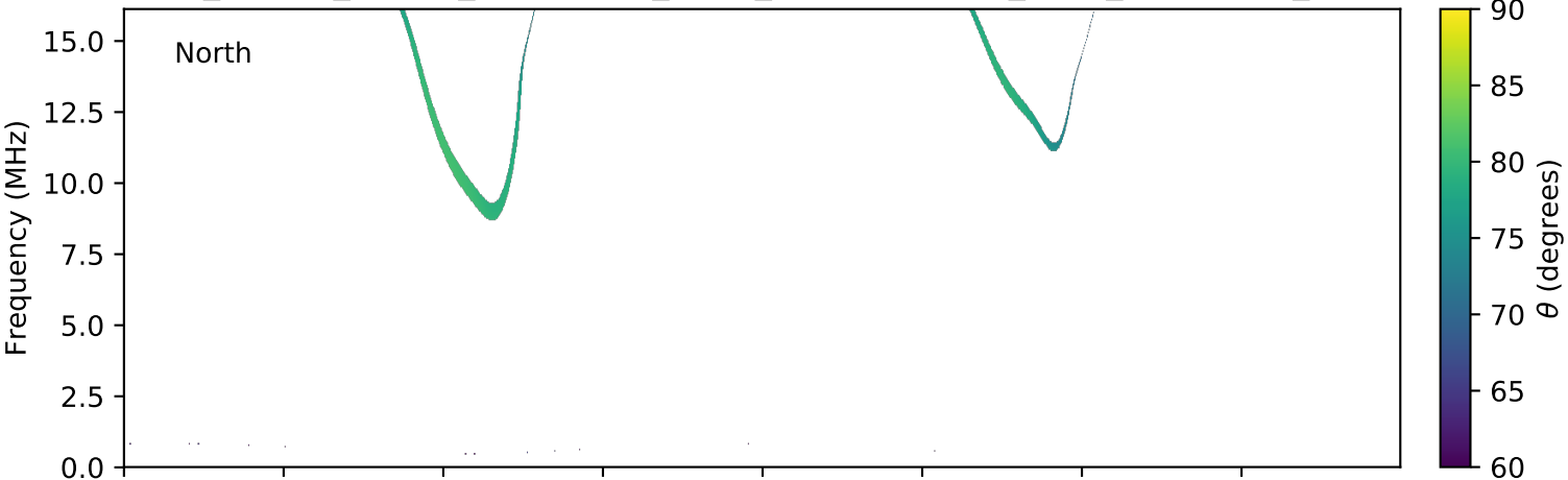
expres_cassini_jupiter_ganymede_isaac_lossc-wid1deg_3kev_20030526_v01.cdf
