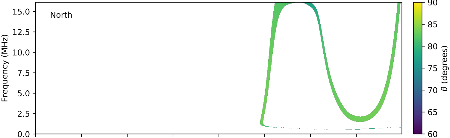
expres_cassini_jupiter_ganymede_isaac_lossc-wid1deg_3kev_20030525_v01.cdf
