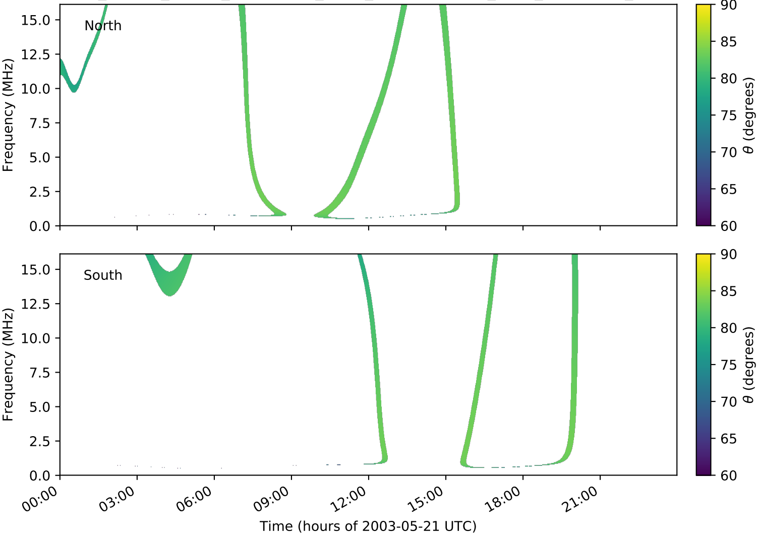
expres_cassini_jupiter_ganymede_isaac_lossc-wid1deg_3kev_20030521_v01.cdf
