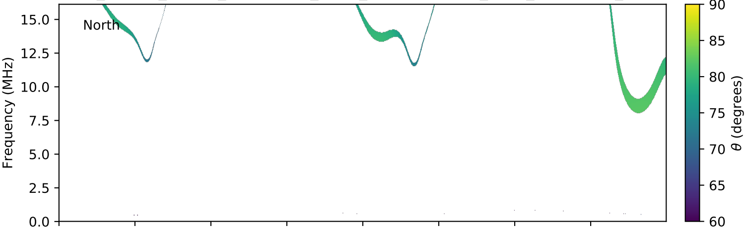
expres_cassini_jupiter_ganymede_isaac_lossc-wid1deg_3kev_20030520_v01.cdf
