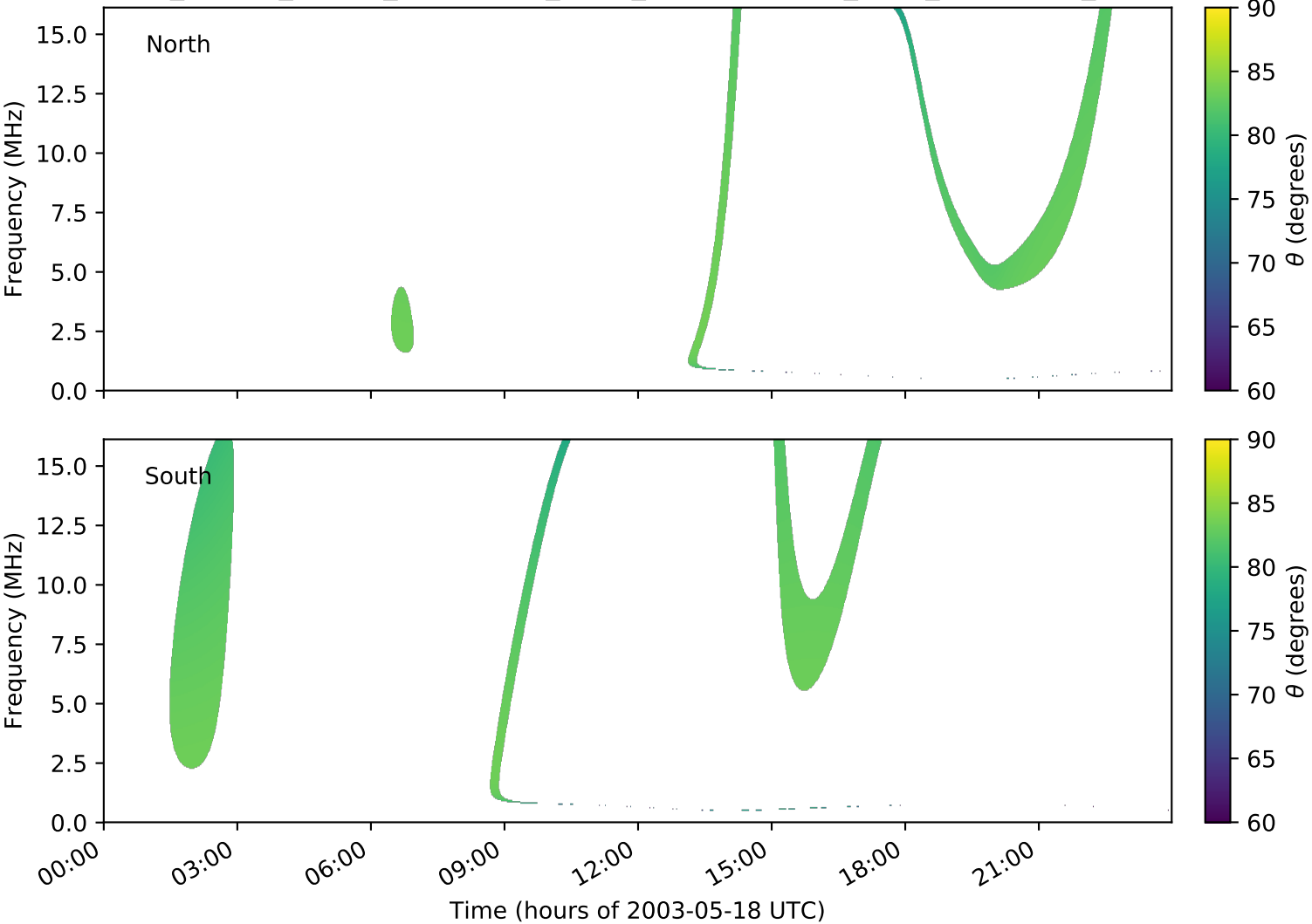
expres_cassini_jupiter_ganymede_isaac_lossc-wid1deg_3kev_20030518_v01.cdf
