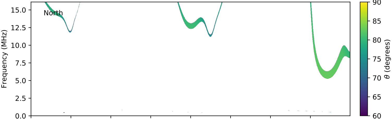
expres_cassini_jupiter_ganymede_isaac_lossc-wid1deg_3kev_20030513_v01.cdf
