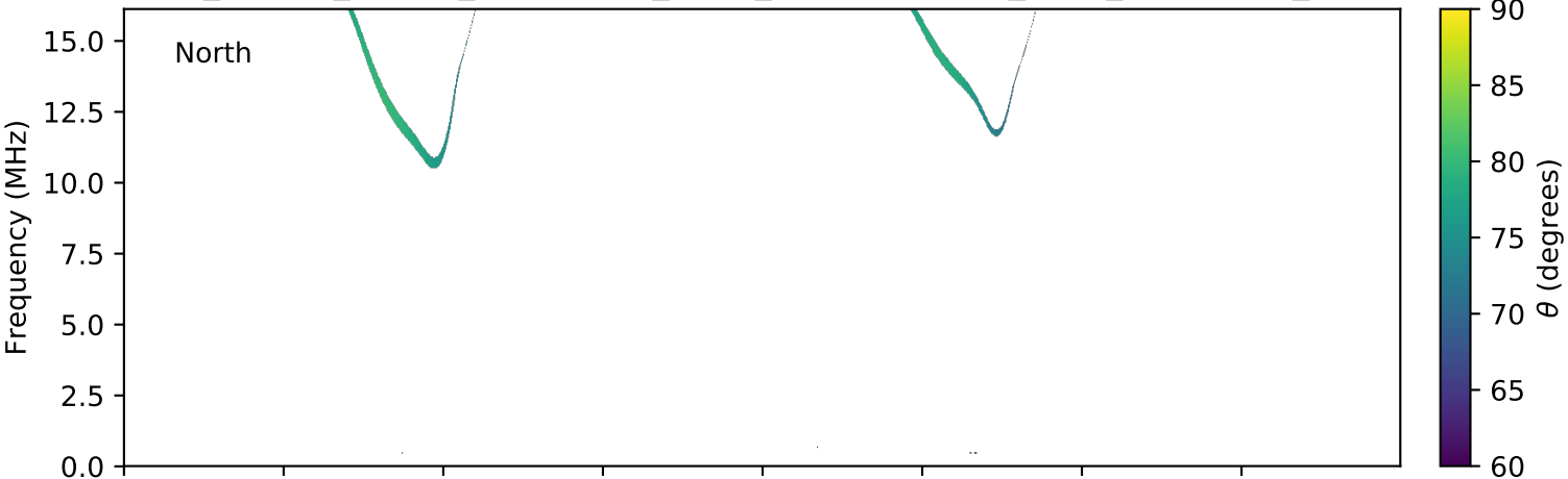
expres_cassini_jupiter_ganymede_isaac_lossc-wid1deg_3kev_20030512_v01.cdf
